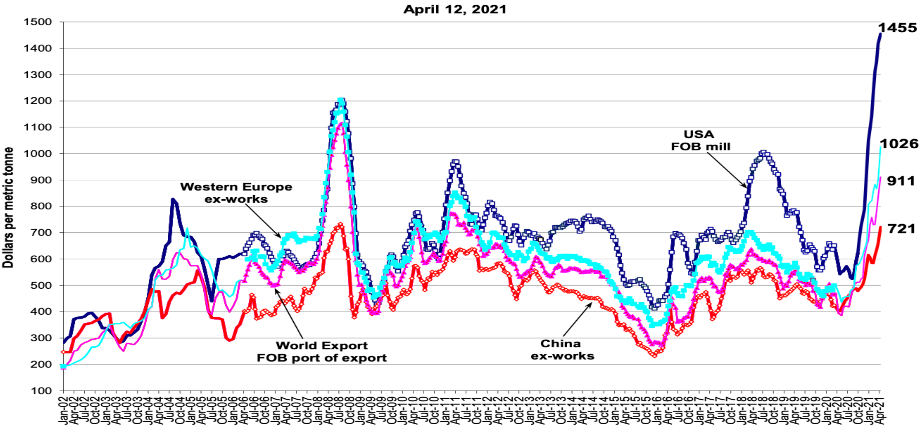
SteelBenchmarker™ HRB Price USA, China, Western Europe and World Export (WSD's PriceTrack data, Jan. 2002 - March 2006; SteelBenchmarker data begins April 2006)
