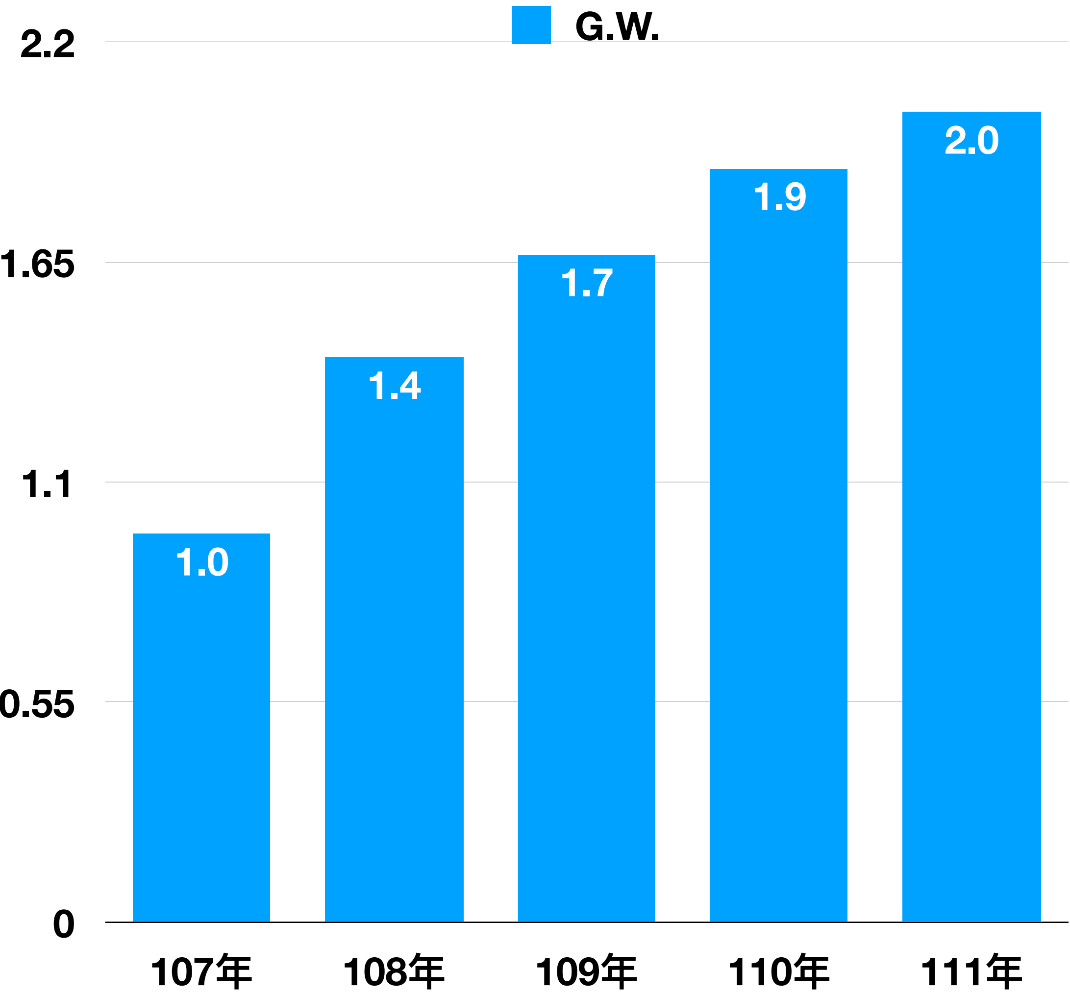
Newly installed capacity of solar power plant in Taiwan every year
